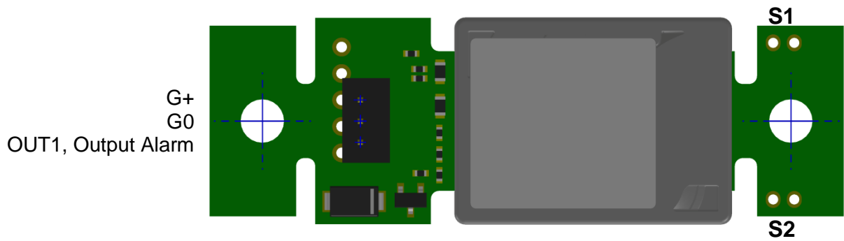
Figure 5. Pin assignment SenseAir ® S8-4B
