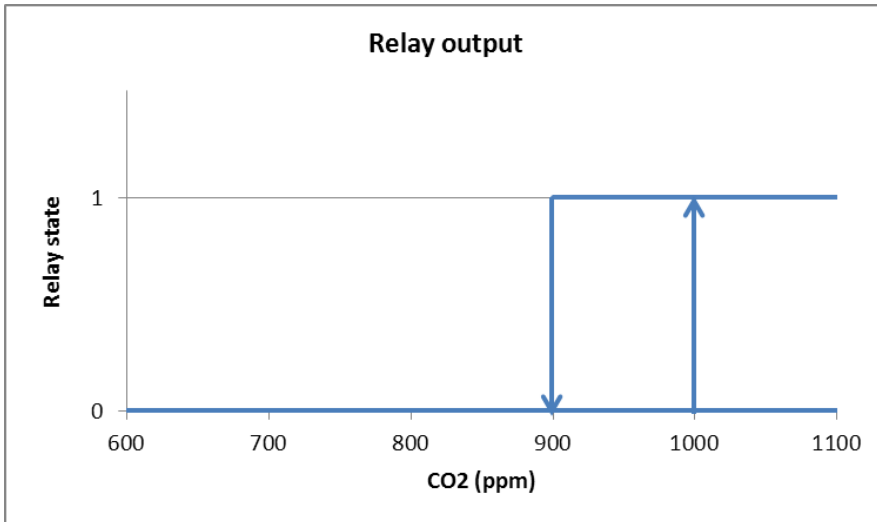
Figure 1, Relay output configured with setpoint = 900 and hysteresis = 100
