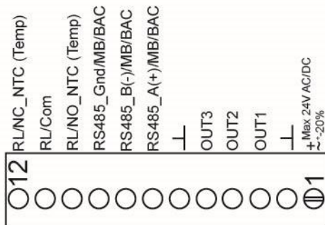
Figure3: Screw Terminal
