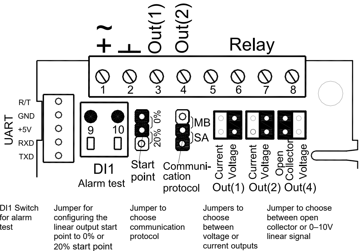
Figure 5 The connection terminal area of the aSENSE MIII with jumpers and terminals. The terminal DI1 may be used for forced ventilation. If the sensor has a heater it is connected to ~ and -.
