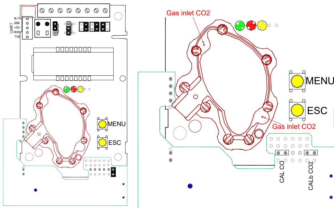
Figure 11 The PCB with the calibration jumper in default position. An enlarged part of the PCB with marked gas inlets and jumper positions for calibration is shown at right.
