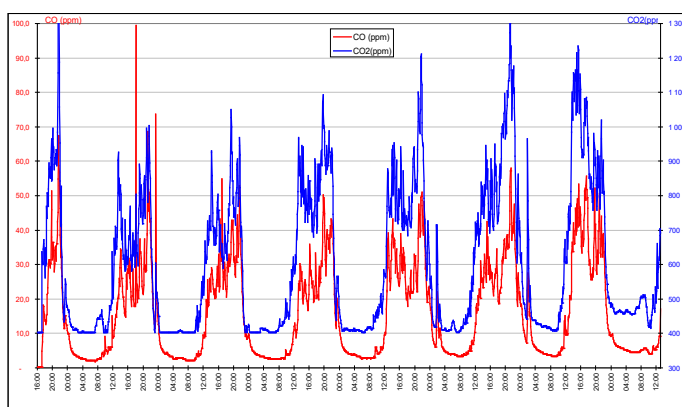
Figure 3 Recorded readings
